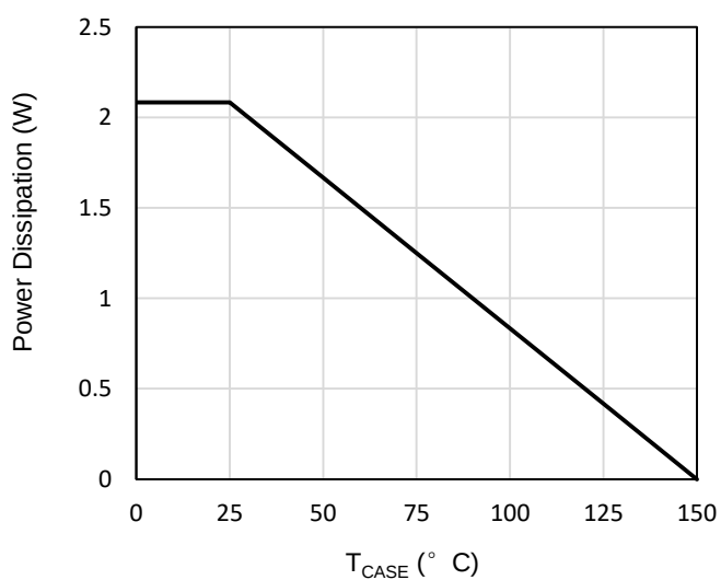
Figure 11: Power De-rating
